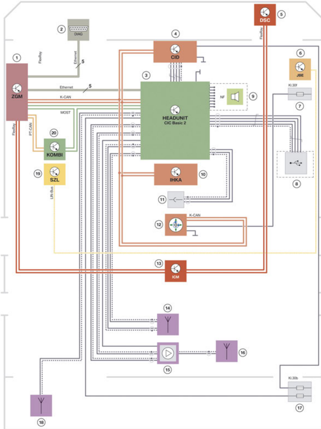
F25 System wiring diagram of CIC Basic 2
