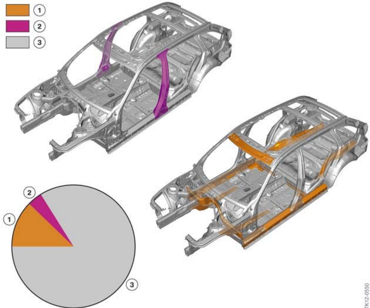
F31 bodyshell, distribution of material grades
